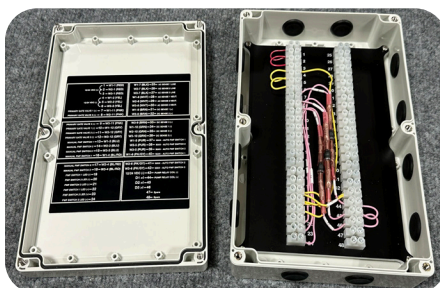
Terminal strips and wiring legend placard in MJM
